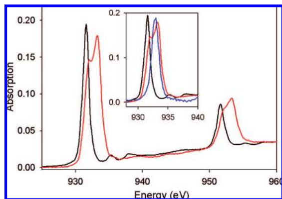
Figure 4. Cu L-edge data of CuSal (black), and [\text{CuSal}]^+ (red). The two major features are the L_3 -edge (ca. 930 eV, 2p_{3/2} \rightarrow 3d_{x^2-y^2} ) and the L_2 -edge (ca. 950 eV, 2p_{1/2} \rightarrow 3d_{x^2-y^2} ). The inset shows the expanded L_3 -edge region for CuSal (black), [\text{CuSal}]^+ (red), and \text{La}_2\text{Li}_{0.5}\text{Cu}_{0.5}\text{O}_4 (blue).
