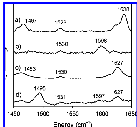
Figure 8. Resonance Raman (rR) spectra of (a) \text{CuSal} and (b) [\text{CuSal}]^+ at 298 K, and of (c) \text{CuSal}^{\text{red}} and (d) [\text{CuSal}^{\text{red}}]^+ at 213 K ( \lambda_{\text{ex}} = 413 \text{ nm} ).
