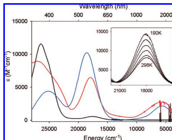
Figure 6. Electronic spectra of 0.08 mM \text{CH}_2\text{Cl}_2 solutions of CuSal (black) and [\text{CuSal}]^+\text{SbF}_6^- (red), and the calculated spectrum for singlet [\text{CuSal}]^+ (blue). Inset: Temperature dependence (298 \rightarrow 190 K) of the 18 000 \text{cm}^{-1} band.
