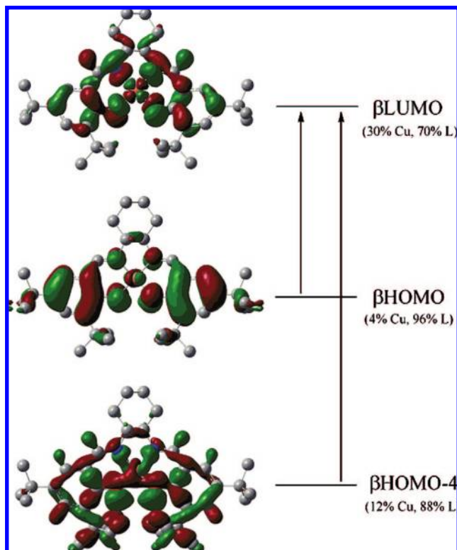
Figure 7. TD-DFT assignment of the calculated transitions for the [\text{CuSal}]^+ singlet state at 18 600 ( \beta\text{HOMO-4} \rightarrow \beta\text{LUMO} ) and 5700 \text{cm}^{-1} ( \beta\text{HOMO} \rightarrow \beta\text{LUMO} ). AOMIX decomposition of relevant MOs into constituent components is shown in parentheses. 42,43
