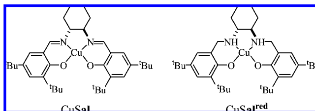
Scheme 2. Structures of CuSal and CuSal red
