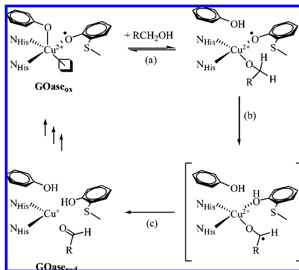
Scheme 1. Consensus Mechanism for the Substrate-Oxidizing Half-Reaction of GOase a
