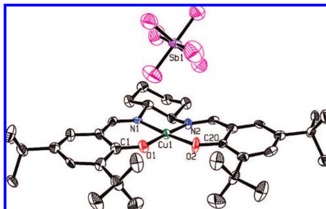
Figure 1. ORTEP representation (50% probability) of [\text{CuSal}]^+\text{SbF}_6^- , excluding hydrogen atoms. Selected interatomic distances (Å) and angles (deg): Cu(1)–O(1), 1.831(6); Cu(1)–O(2), 1.838(6); Cu(1)–N(1), 1.877(6); Cu(1)–N(2), 1.880(6); N(1)–C(7), 1.290(9); N(2)–C(14), 1.292(10); O(1)–C(1), 1.317(10); O(2)–C(20), 1.317(9); O(1)–Cu(1)–O(2), 86.5(3); O(1)–Cu(1)–N(1), 94.3(3); O(2)–Cu(1)–N(2), 93.8(3); N(1)–Cu(1)–N(2), 85.7(3).
