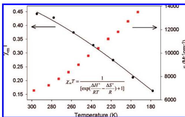
Figure 9. Comparison of the VT solution susceptibility by ^1\text{H} NMR (black circles, \text{CD}_2\text{Cl}_2 ) and 18 000 \text{cm}^{-1} band intensity (red squares, \text{CH}_2\text{Cl}_2 ) for [\text{CuSal}]^+\text{SbF}_6^- . Fitting the susceptibility values (solid line) to the equation indicated affords thermodynamic parameters for the equilibrium ( \Delta H^\circ = 1.1 \pm 0.1 \text{ kcal mol}^{-1} , \Delta S^\circ = 3.5 \pm 0.1 \text{ cal K}^{-1} \text{ mol}^{-1} ; R^2 = 0.998 ).
