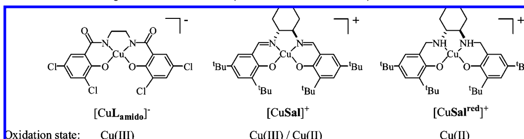
Scheme 4. Metal Oxidation State Assignment for a Series of Square-Planar Cu–N 2 O 2 Complexes a
