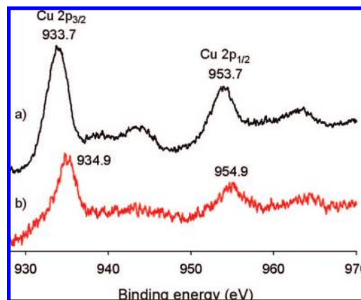
Figure 5. X-ray photoelectron spectroscopy (XPS) data for CuSal (a) and [\text{CuSal}]^+ (b).
